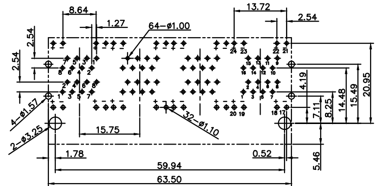
PC Board Layout Component Side Shown PC Board Thickness=1.6mm Tolerance \pm 0.05
